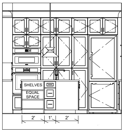
K5 ISLAND LEFT 3/16 in = 1 ft
