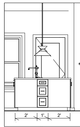
K6 ISLAND RIGHT 3/16 in = 1 ft
