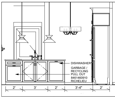
K4 KITCHEN ISLAND 3/16 in = 1 ft
